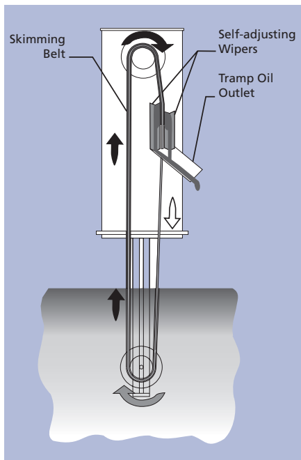
Model 8A Oil Recovery Unit
